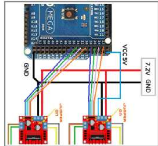
Figure 4.7 Arduino Mega Wiring Relations With the L298 Motorcycle Driver (Source: Self-processed Results)
