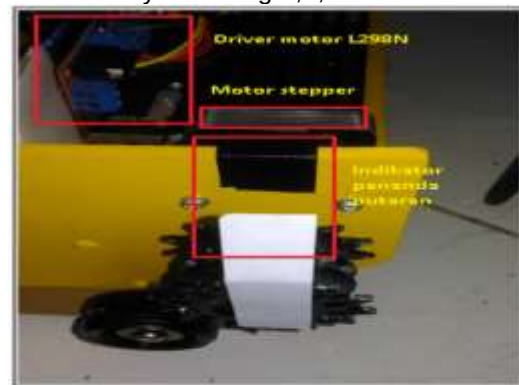
Figure 4. 9 Motor Rotational Testing (Source: Self-processed Results)
