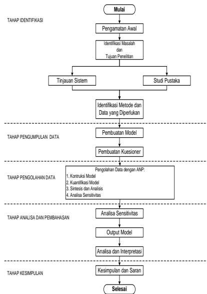
Gambar 3.1 Flowchart Penelitian
