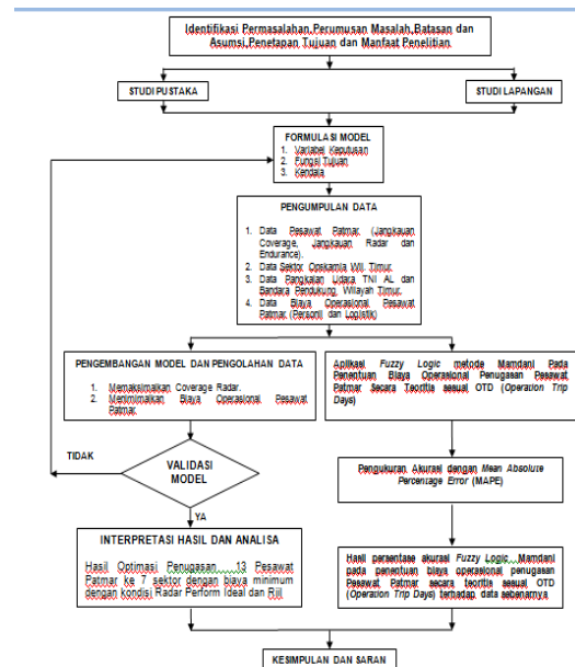
Gambar 3.1 Flowchart Penelitian
